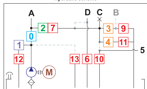
Hydraulic scheme
