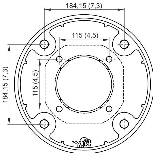
Adaptor flange
