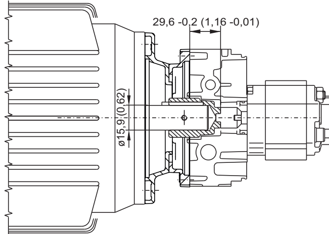
Couplings
