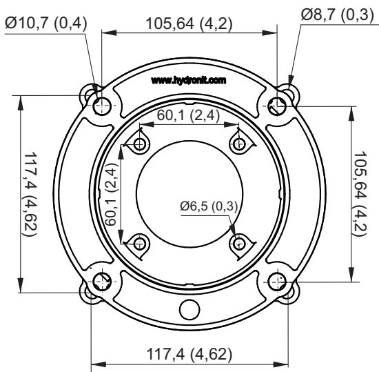
Adaptor flange
