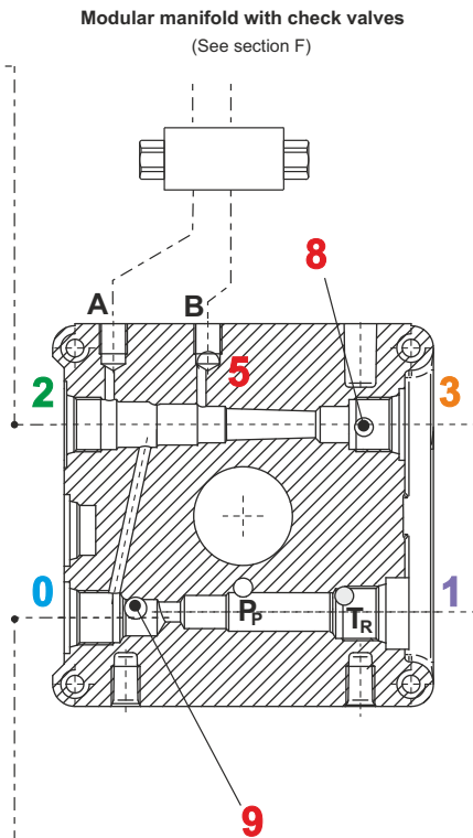
Hydraulic scheme
